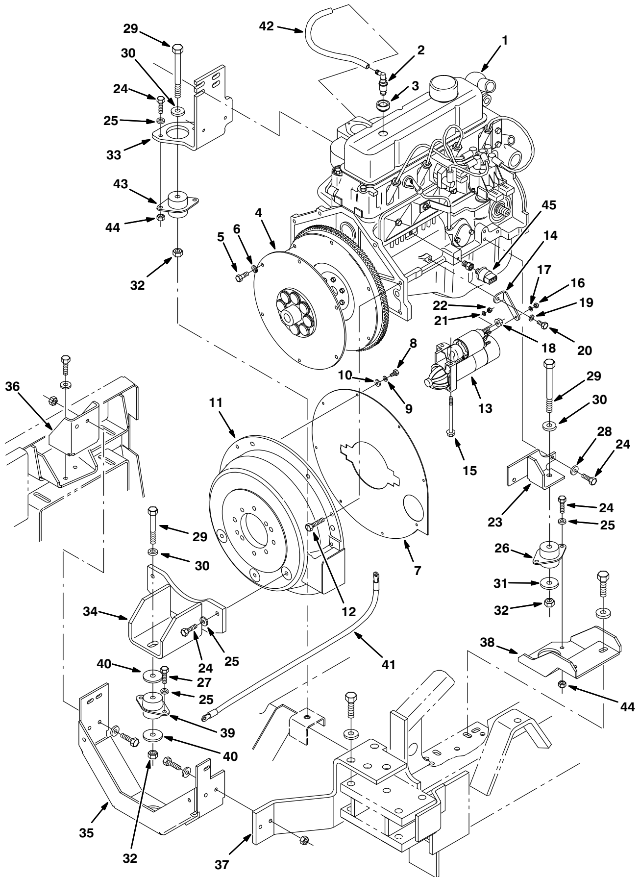
Fig. 22 – Engine Group (004937–005999)
