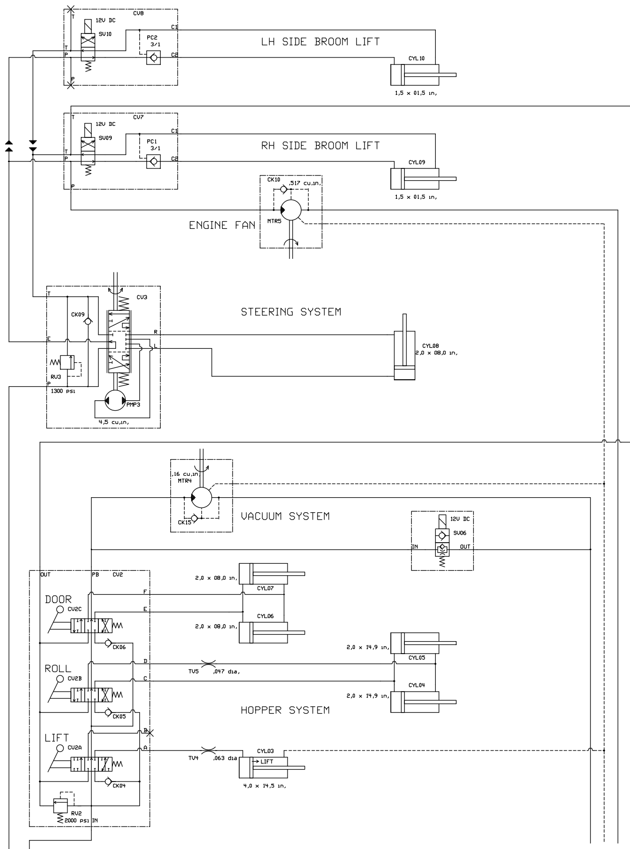
Fig. 74 – Hydraulic Schematic
