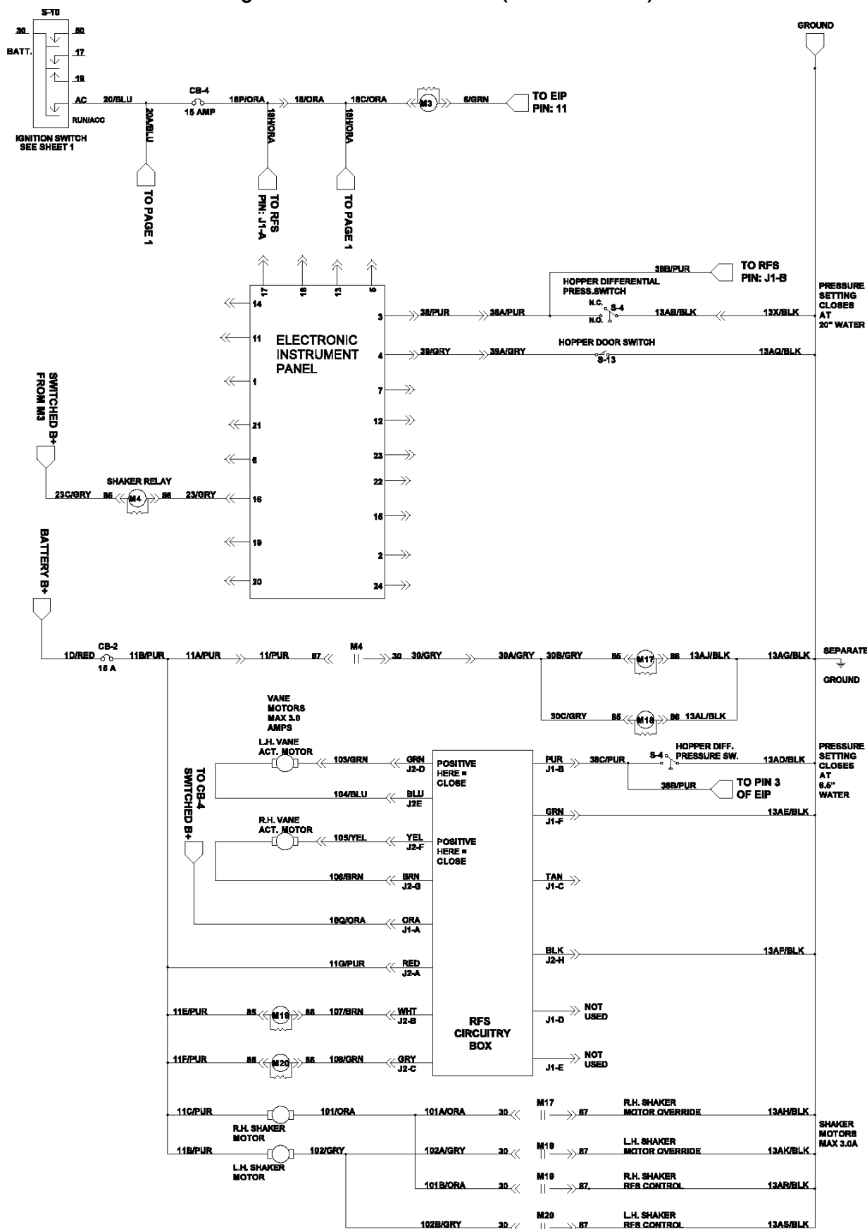
Fig. 93 – Electrical Schematic (004937–005999)
