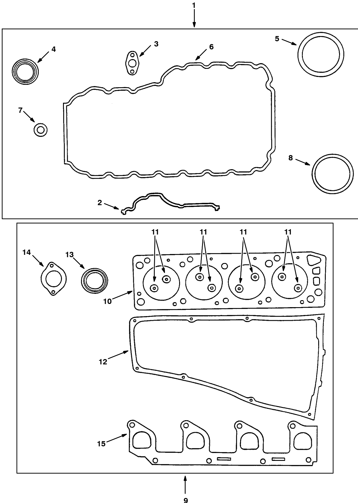
Fig. 2 - Gaskets Group
