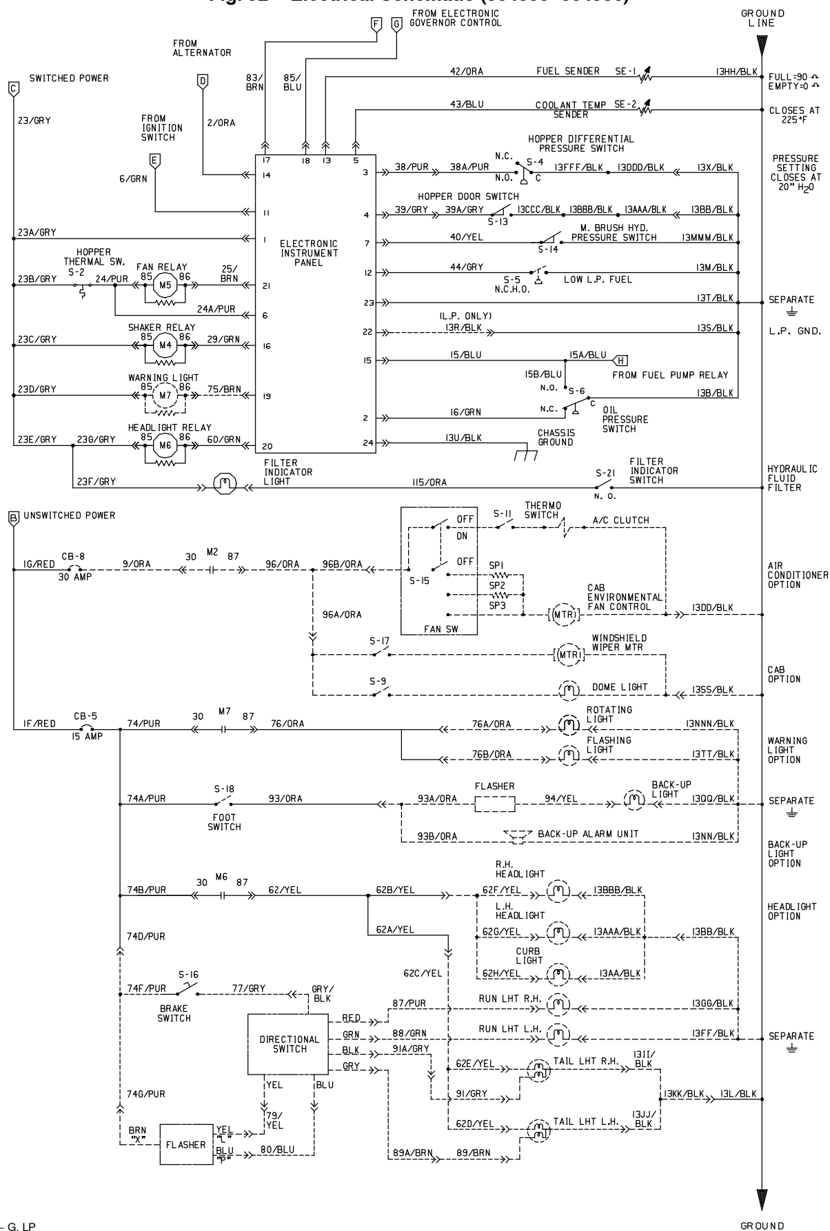
Fig. 92 – Electrical Schematic (004000–004936)
