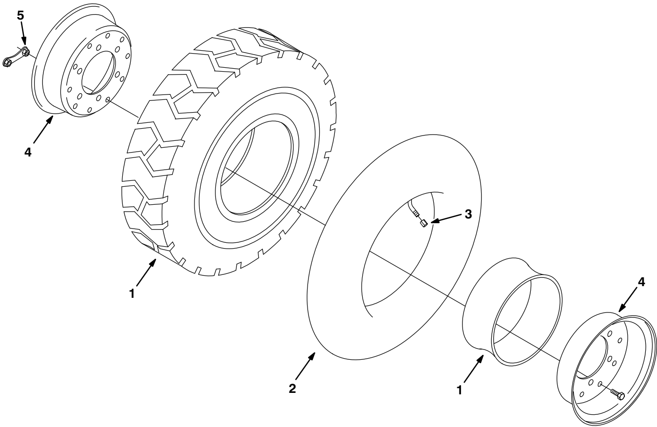
Fig. 70 – Wheel Assembly
