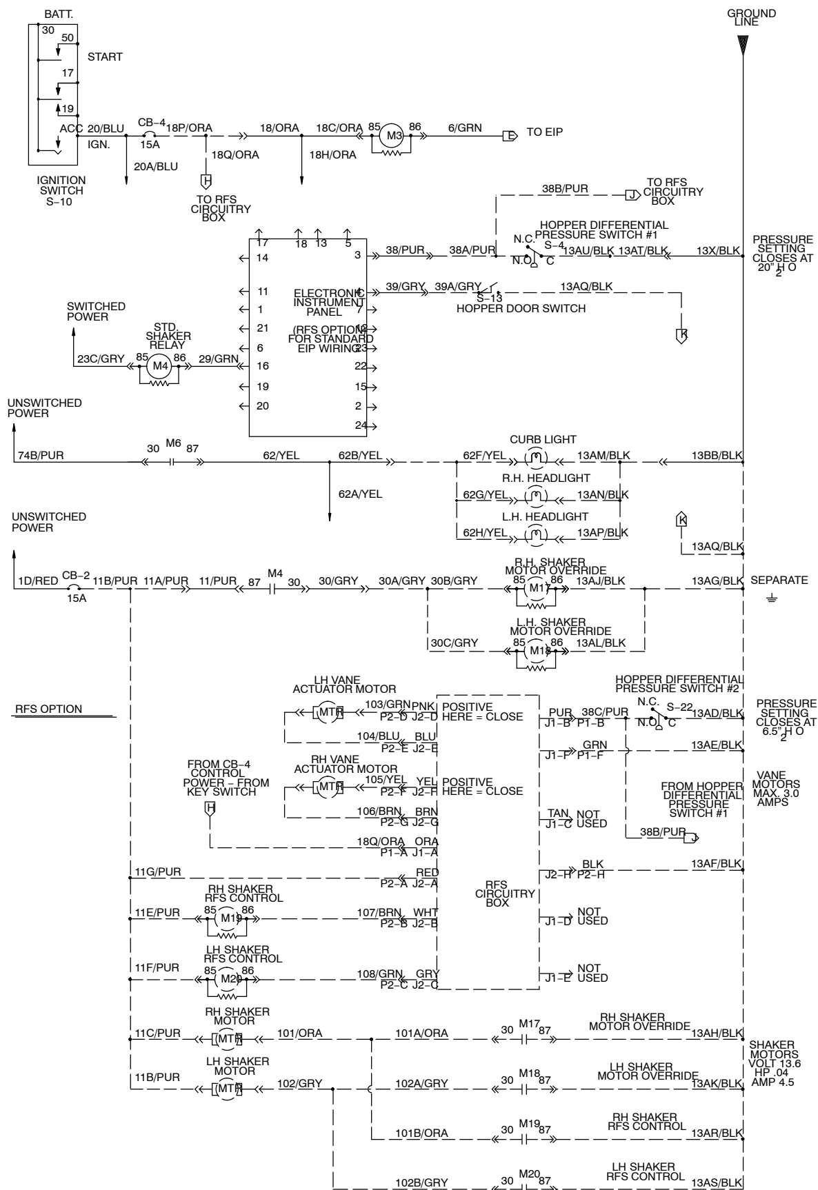
Fig. 92 – Electrical Schematic (004000-004936)
