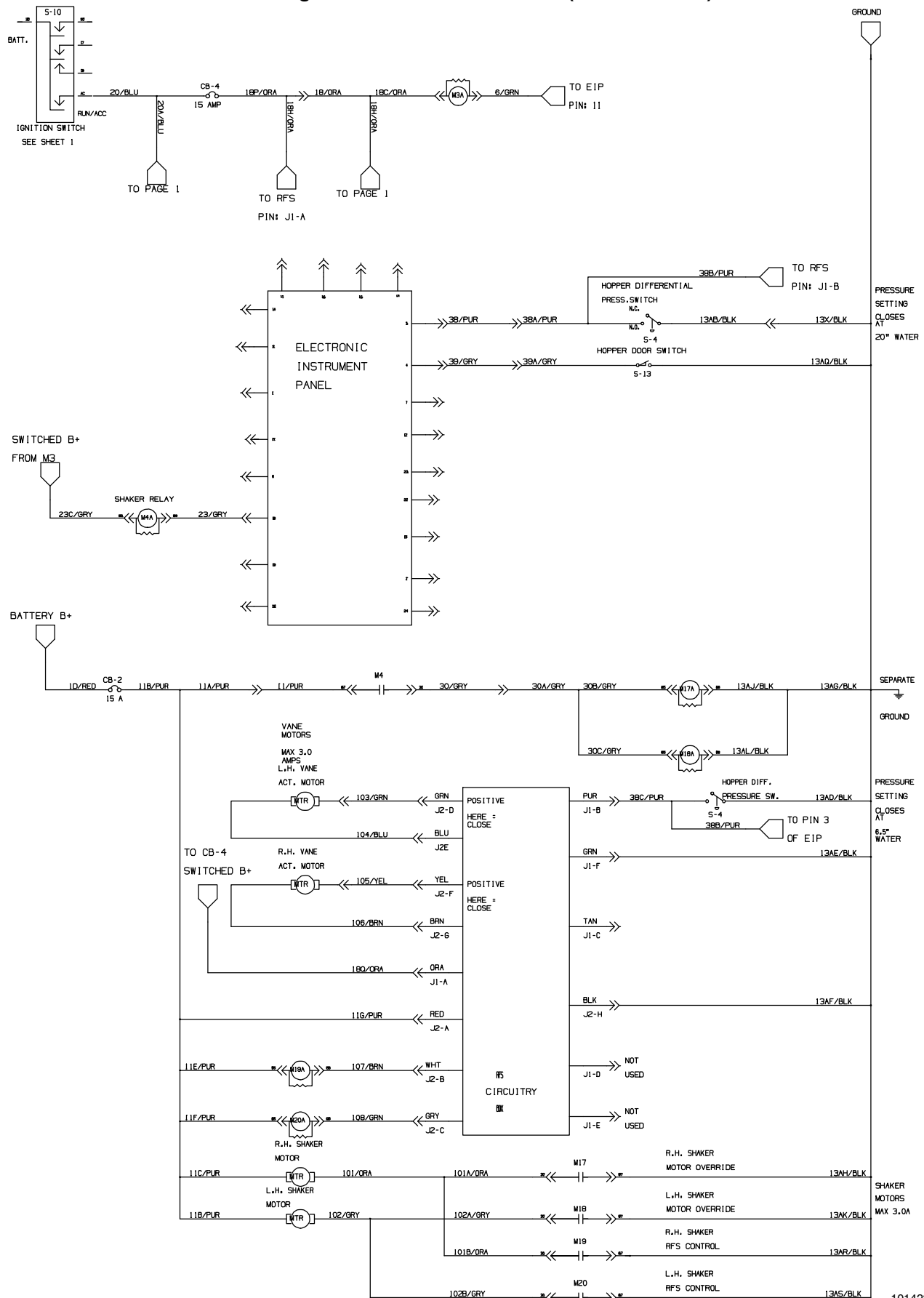
Fig. 94 – Electrical Schematic (006000- )
