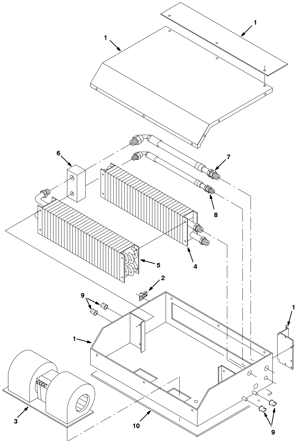
Fig. 34 – AC and Heater Box Breakdown, 380613 (000000–008088)
