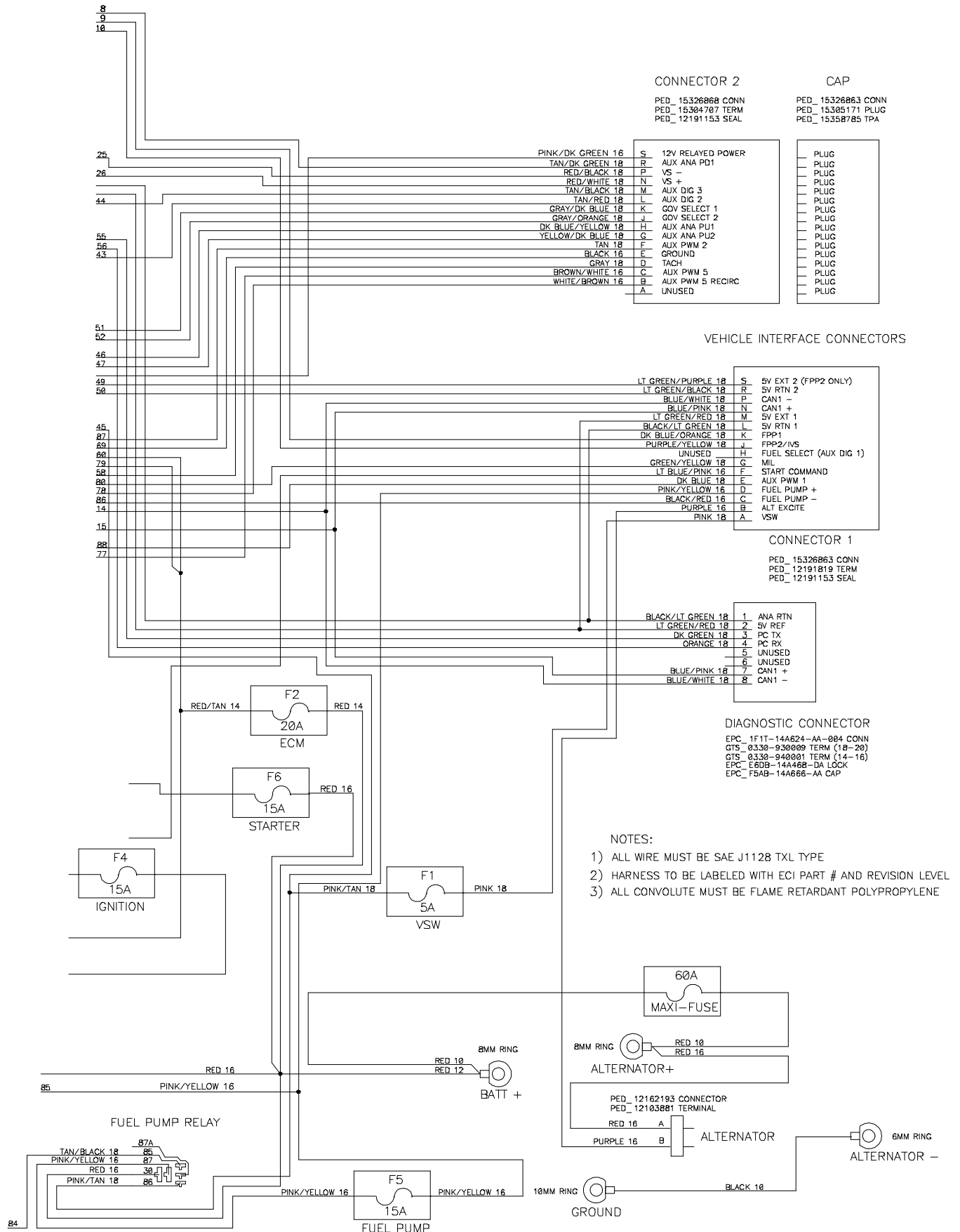
Fig. 104 – Wire Harnesses Schematic, Gas Engine (007000– )
