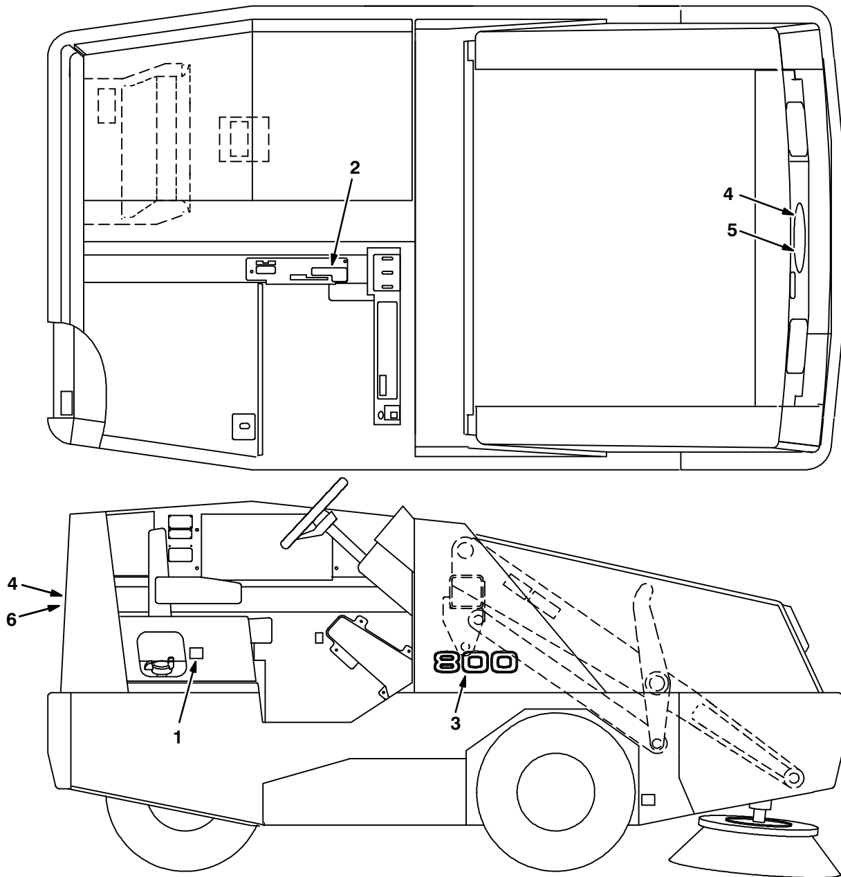
Fig. 108 – Label Group
