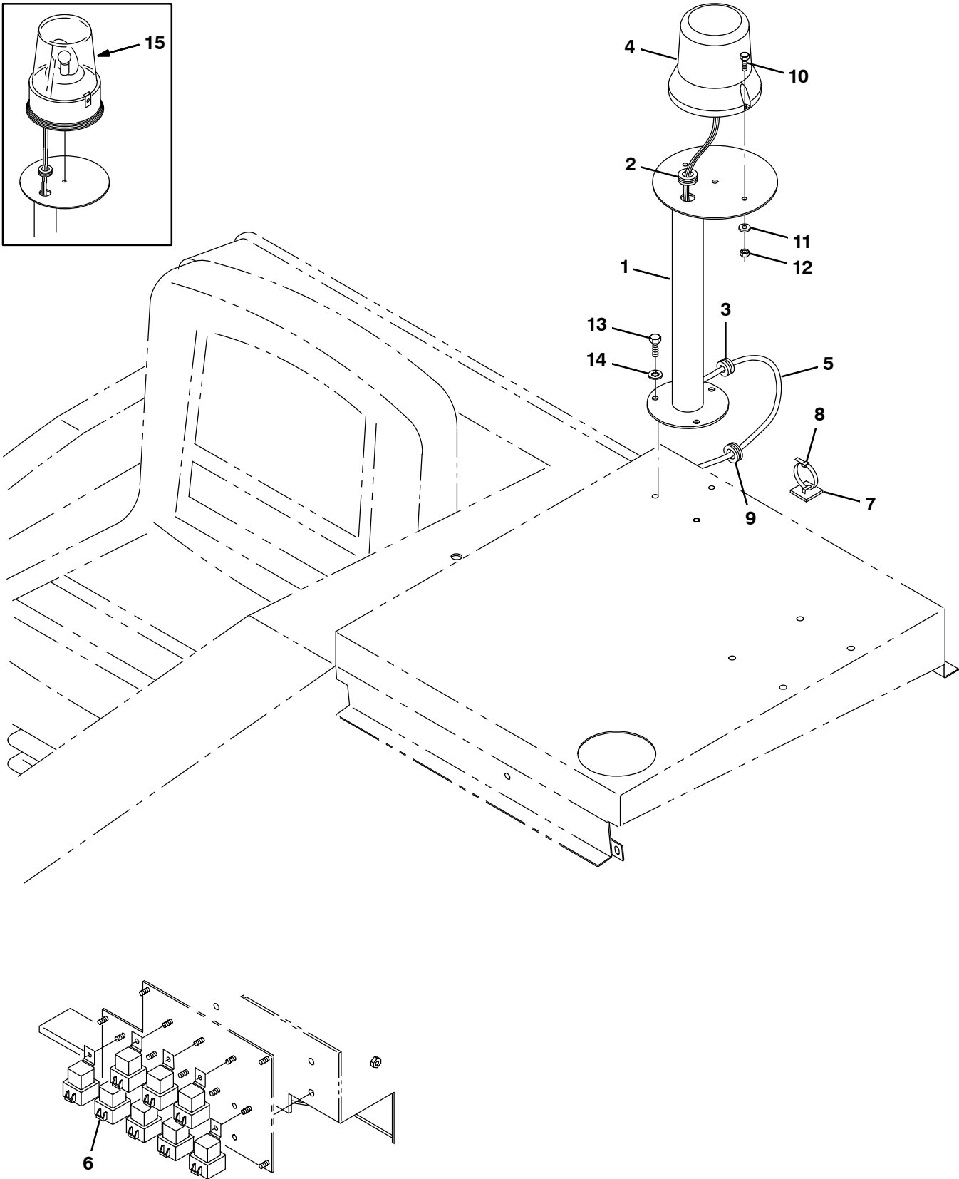
Fig. 11 – Light Kit, Strobe, Low (004000–008088)
