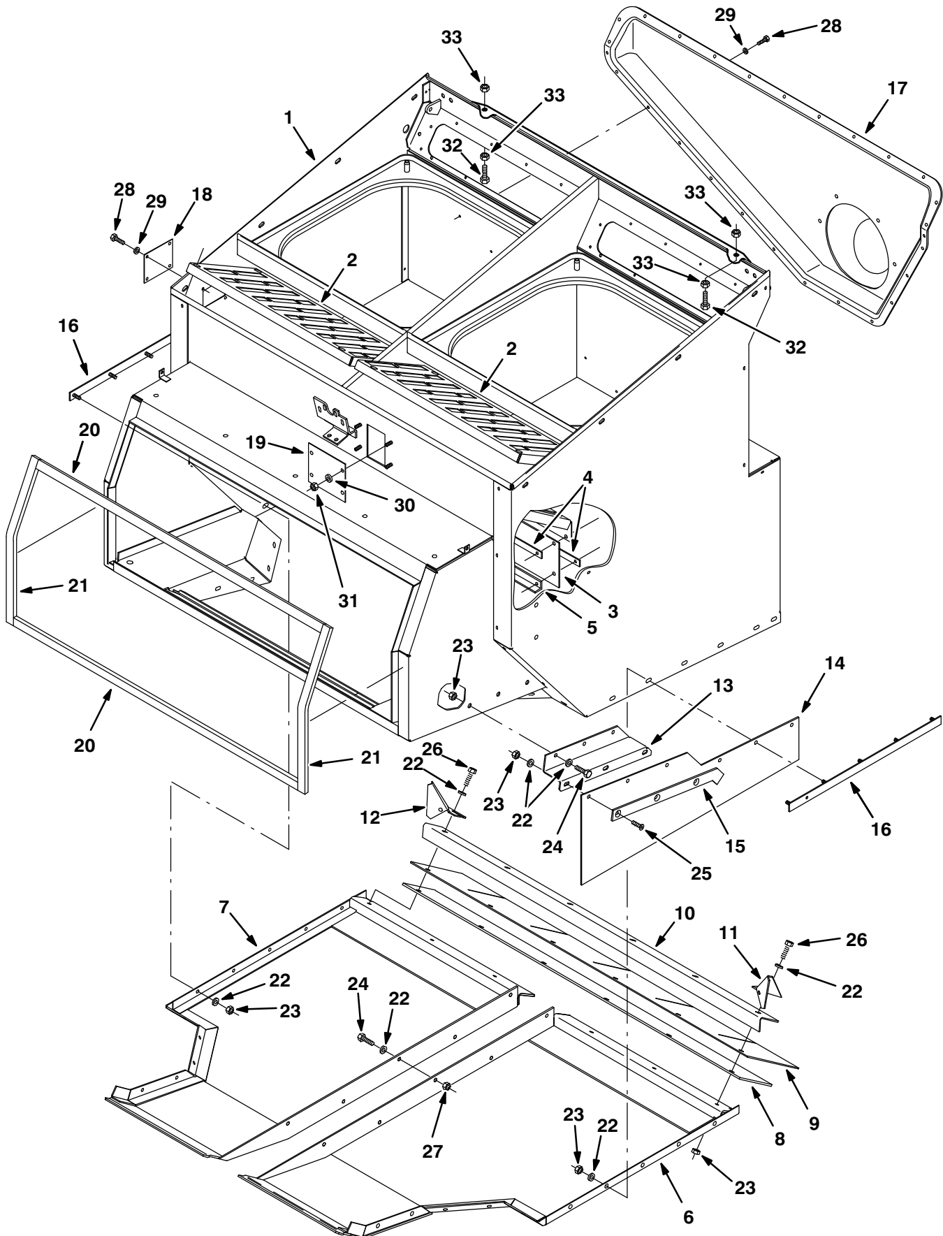
Fig. 14 – Hopper Group
