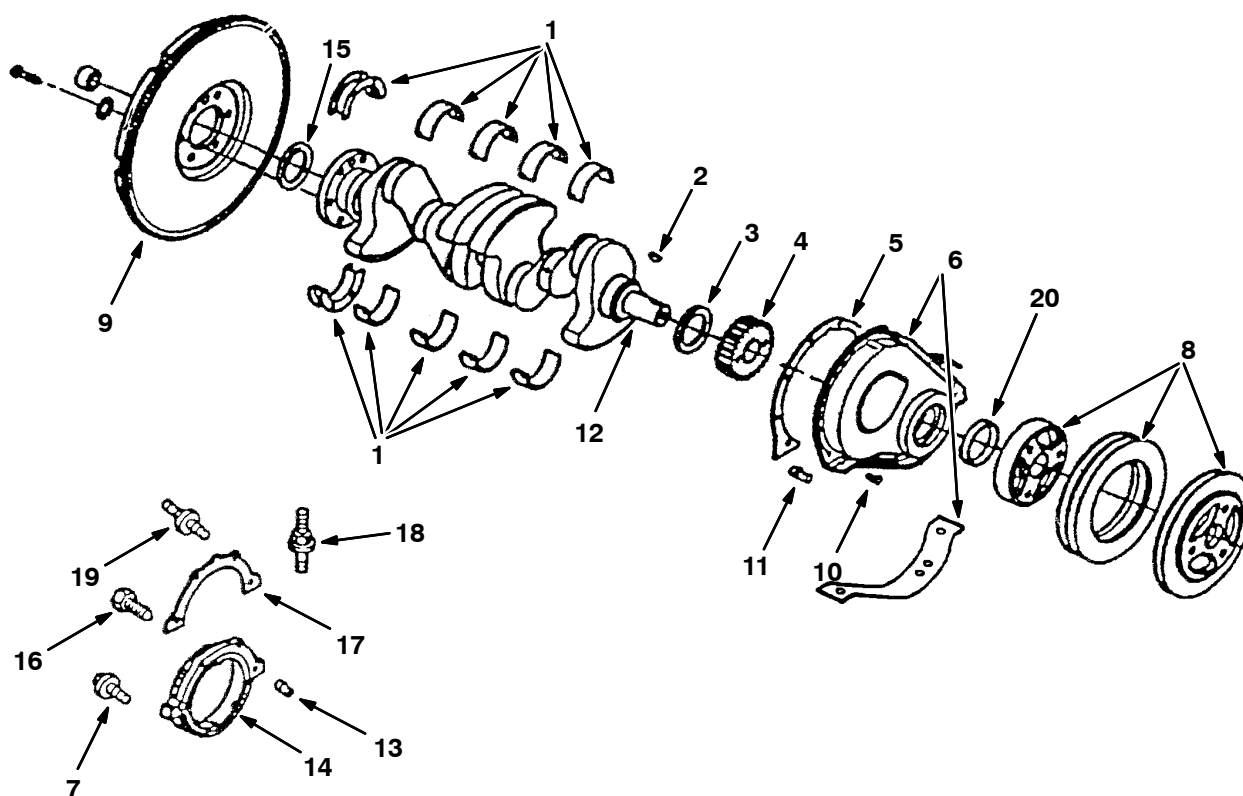
Fig. 5 – Crankshaft Group
