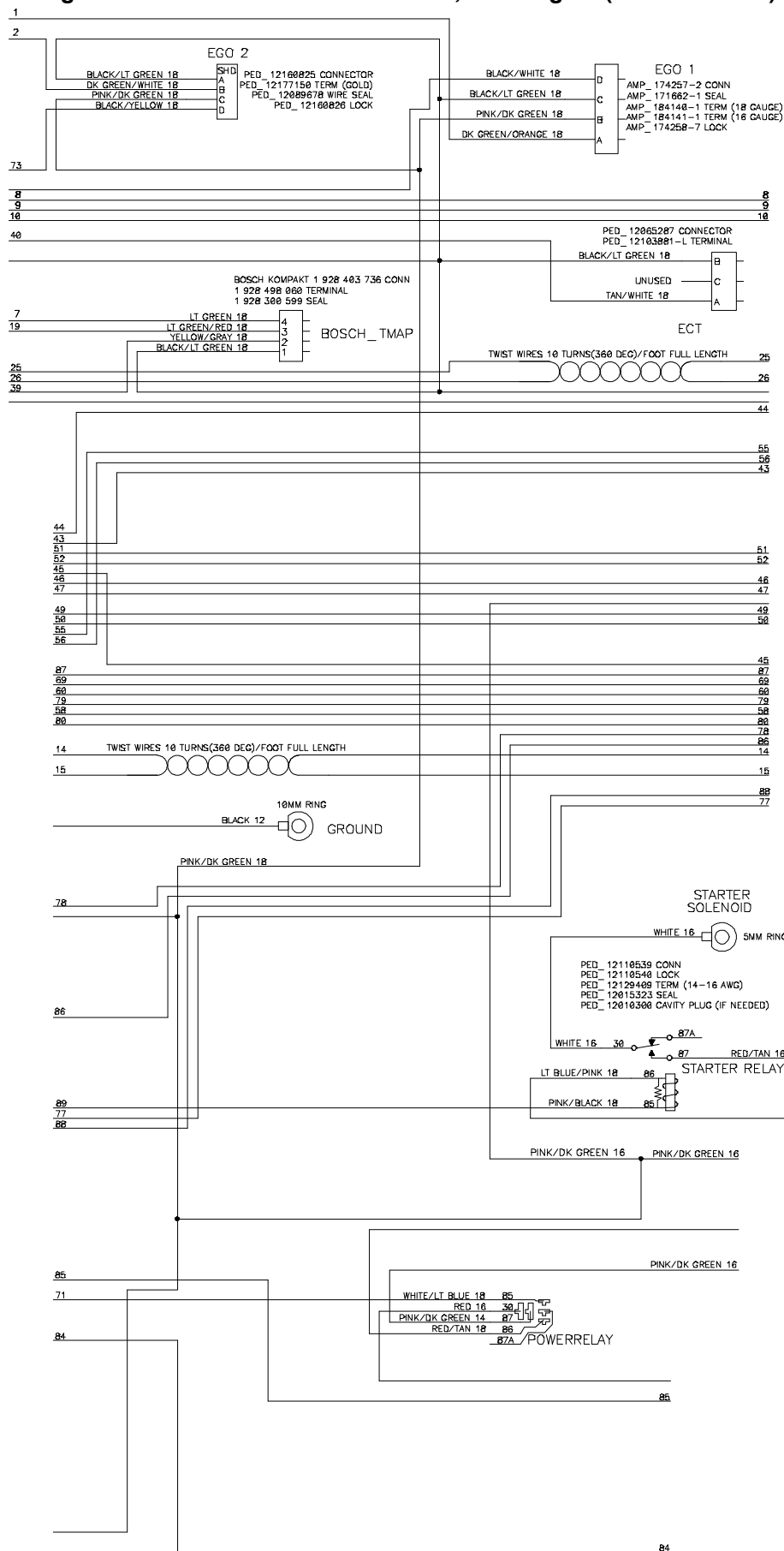
Fig. 104 – Wire Harnesses Schematic, Gas Engine (007000– )
