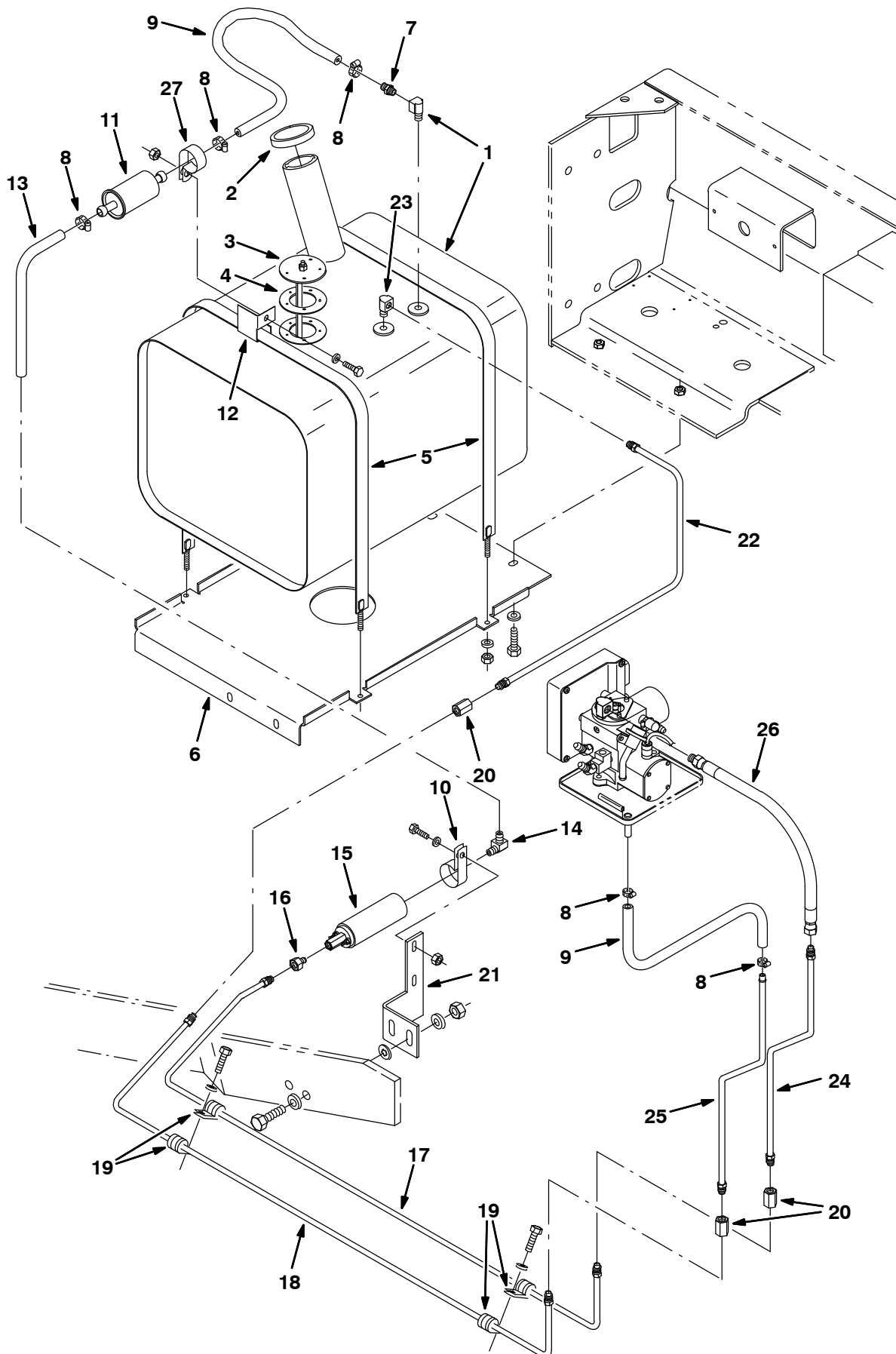
Fig. 52 – Engine Fuel Tank Group, Gas (004937–005999)
