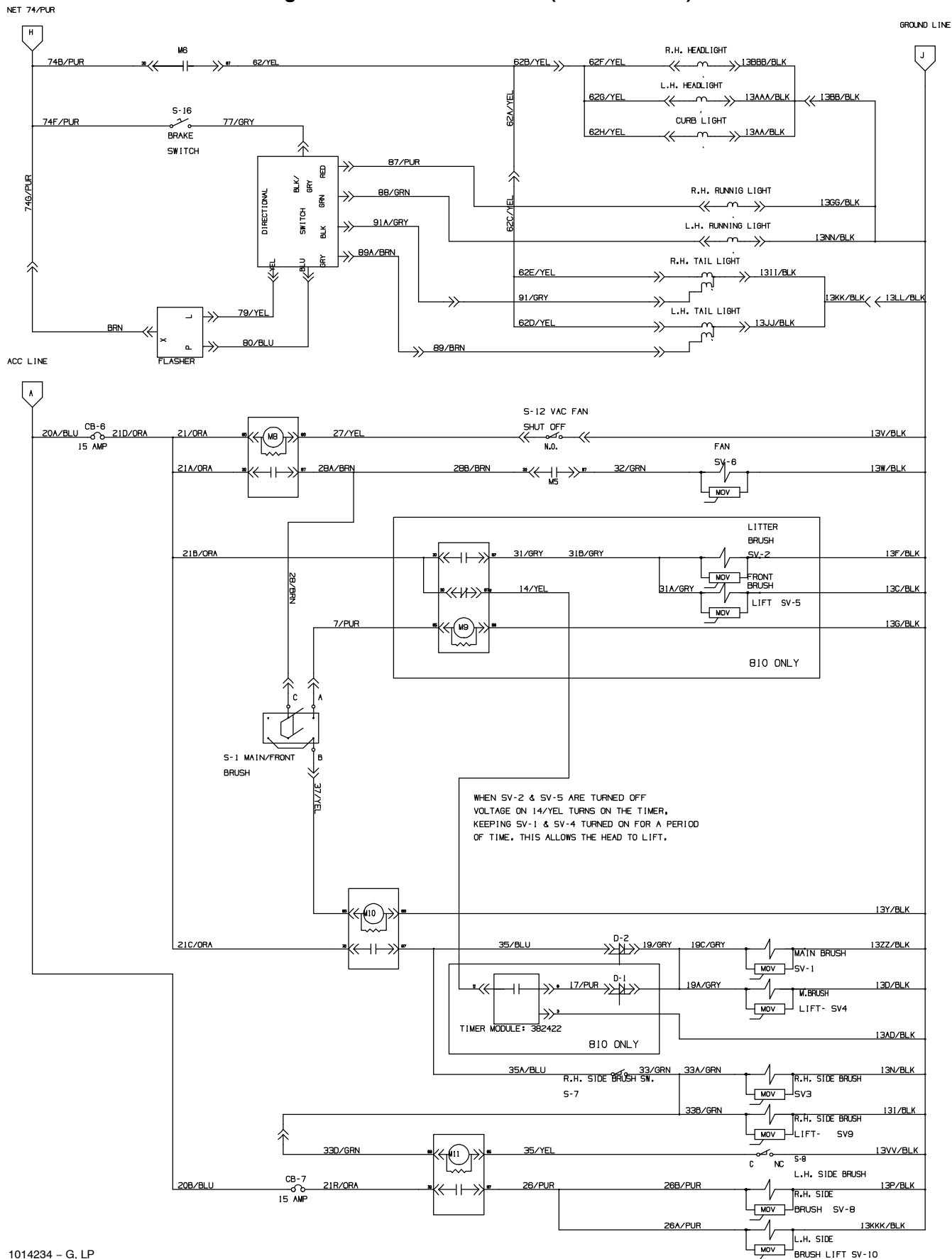
Fig. 94 – Electrical Schematic (006000- )
