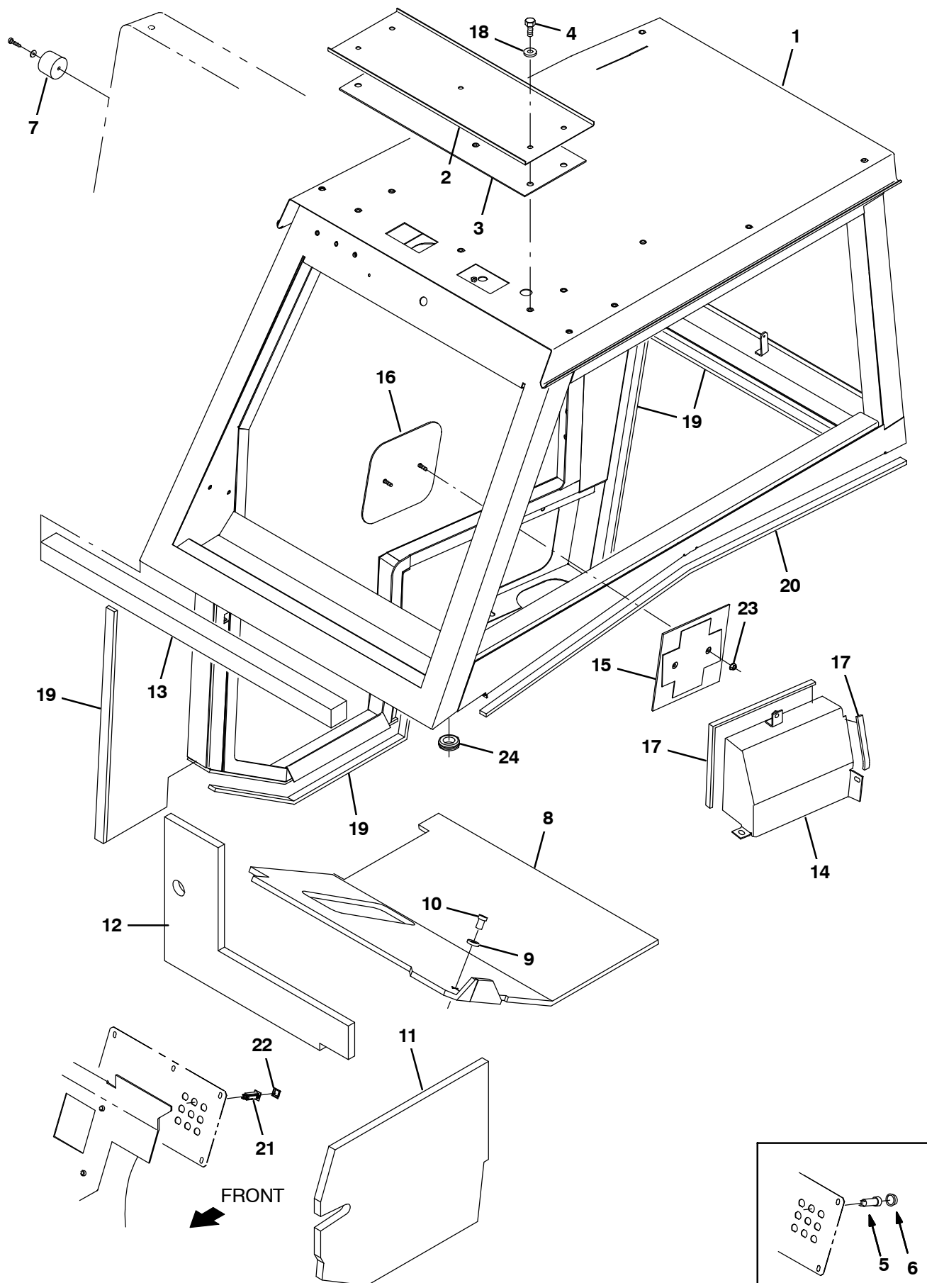
Fig. 29 – Cab Kit
