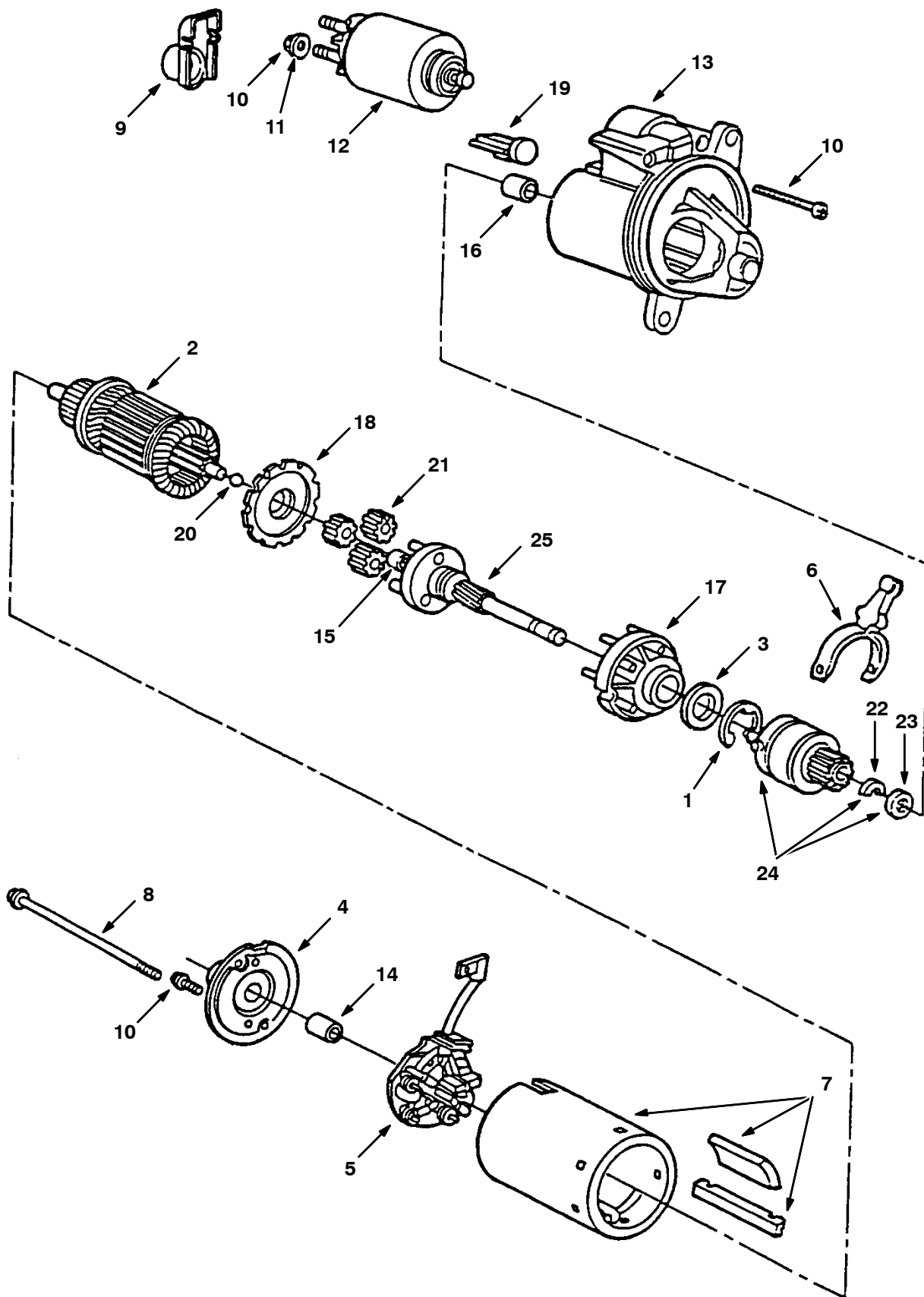
Fig. 5 – Starter Breakdown
