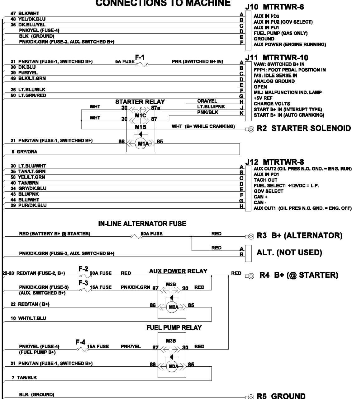
Fig. 94 – Electrical Schematic (006000– )
