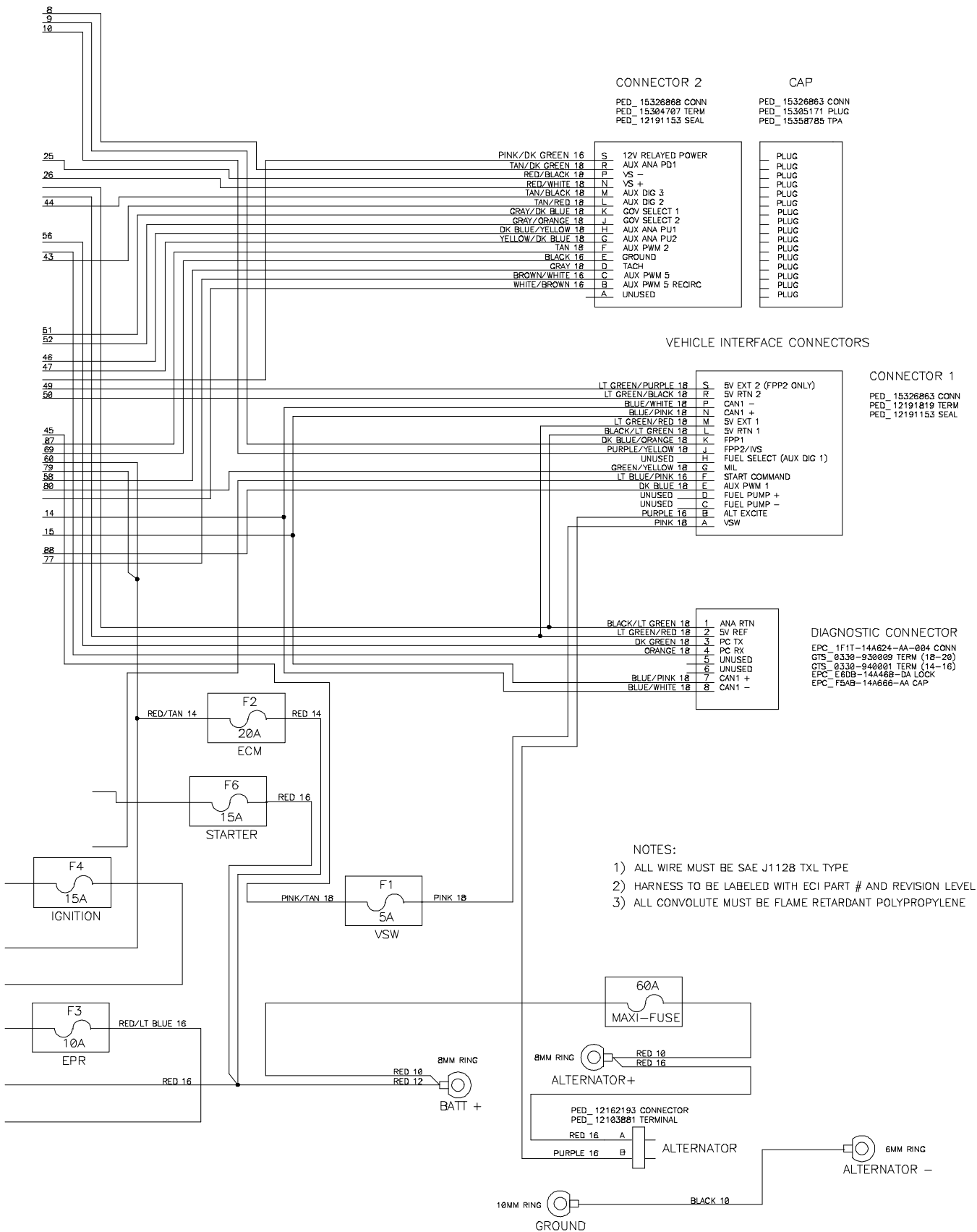
Fig. 105 – Wire Harnesses Schematic, LPG Engine (007000– )
