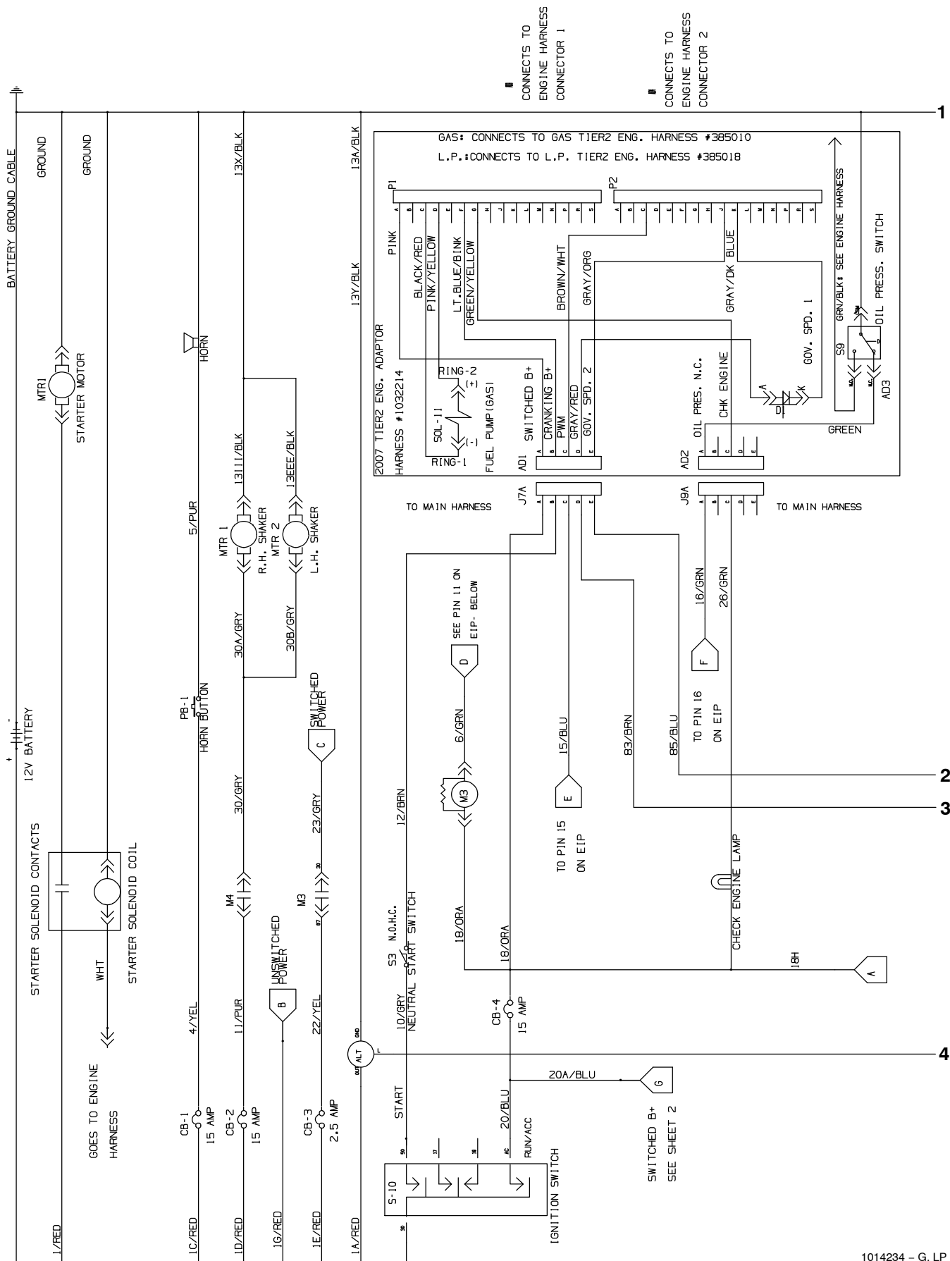
Fig. 94 – Electrical Schematic (006000– )
