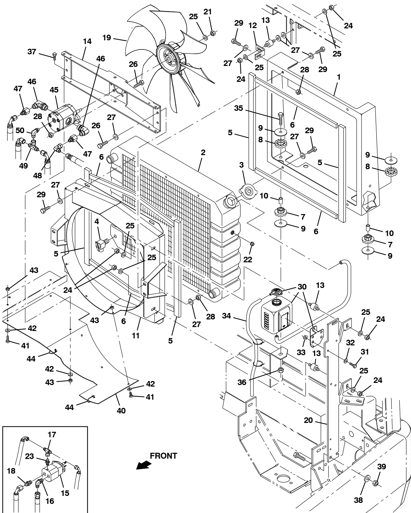
Fig. 65 – Engine Radiator and Cooling Fan Group (007000– )
