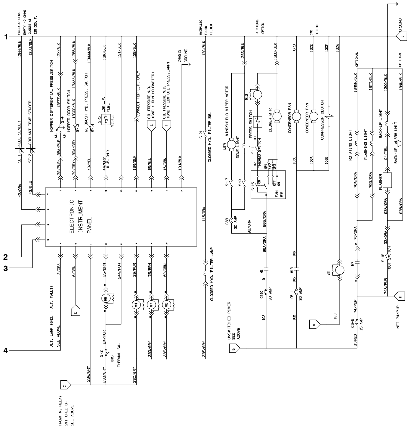
Fig. 94 – Electrical Schematic (006000– )
