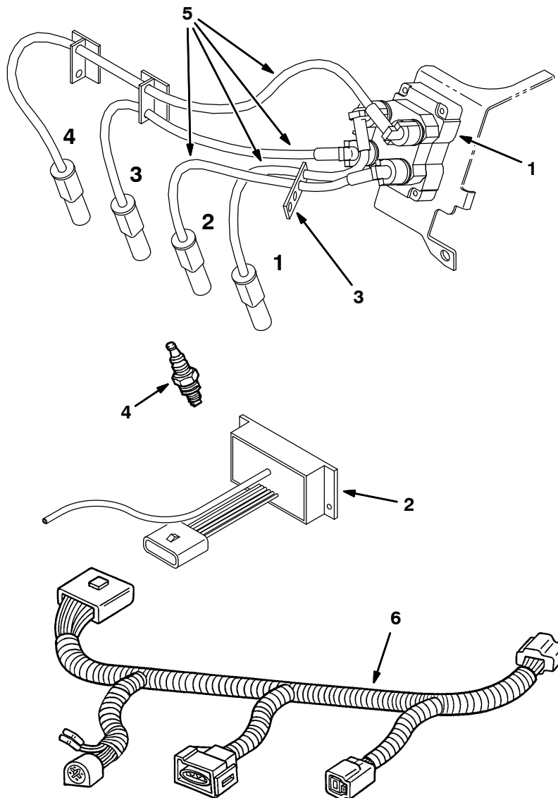
Fig. 14 – Ignition Group
