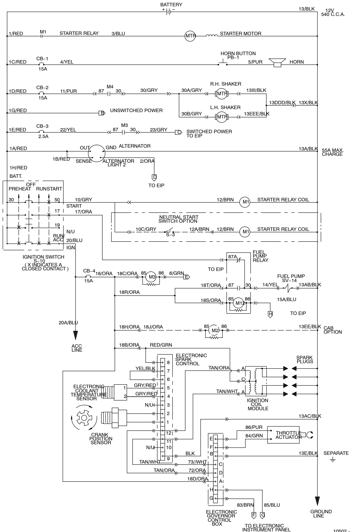
Fig. 92 – Electrical Schematic (004000–004936)
