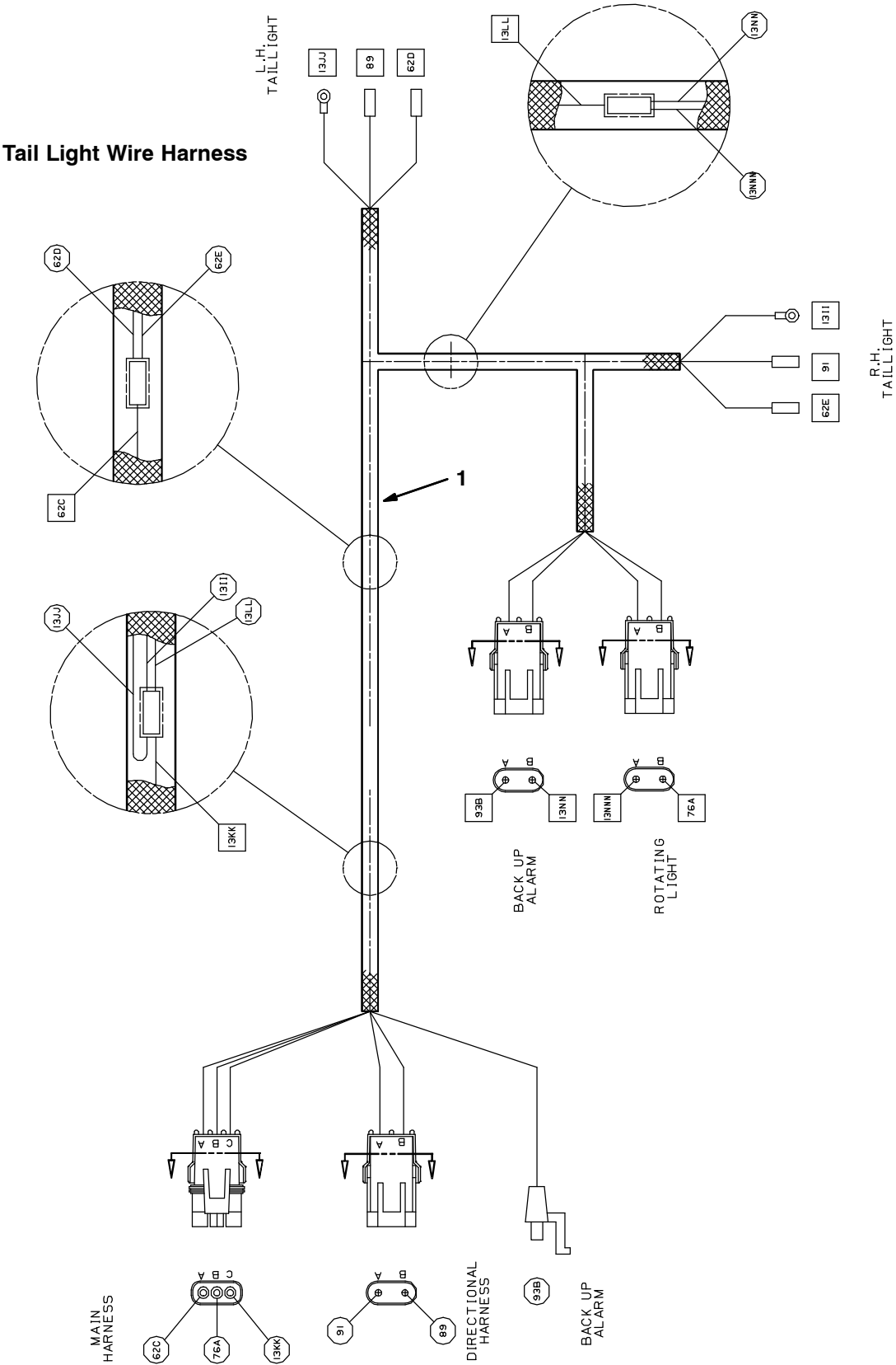
Fig. 97 – Wire Harnesses Group, Gas/LPG, Tail Lights (004000– )
