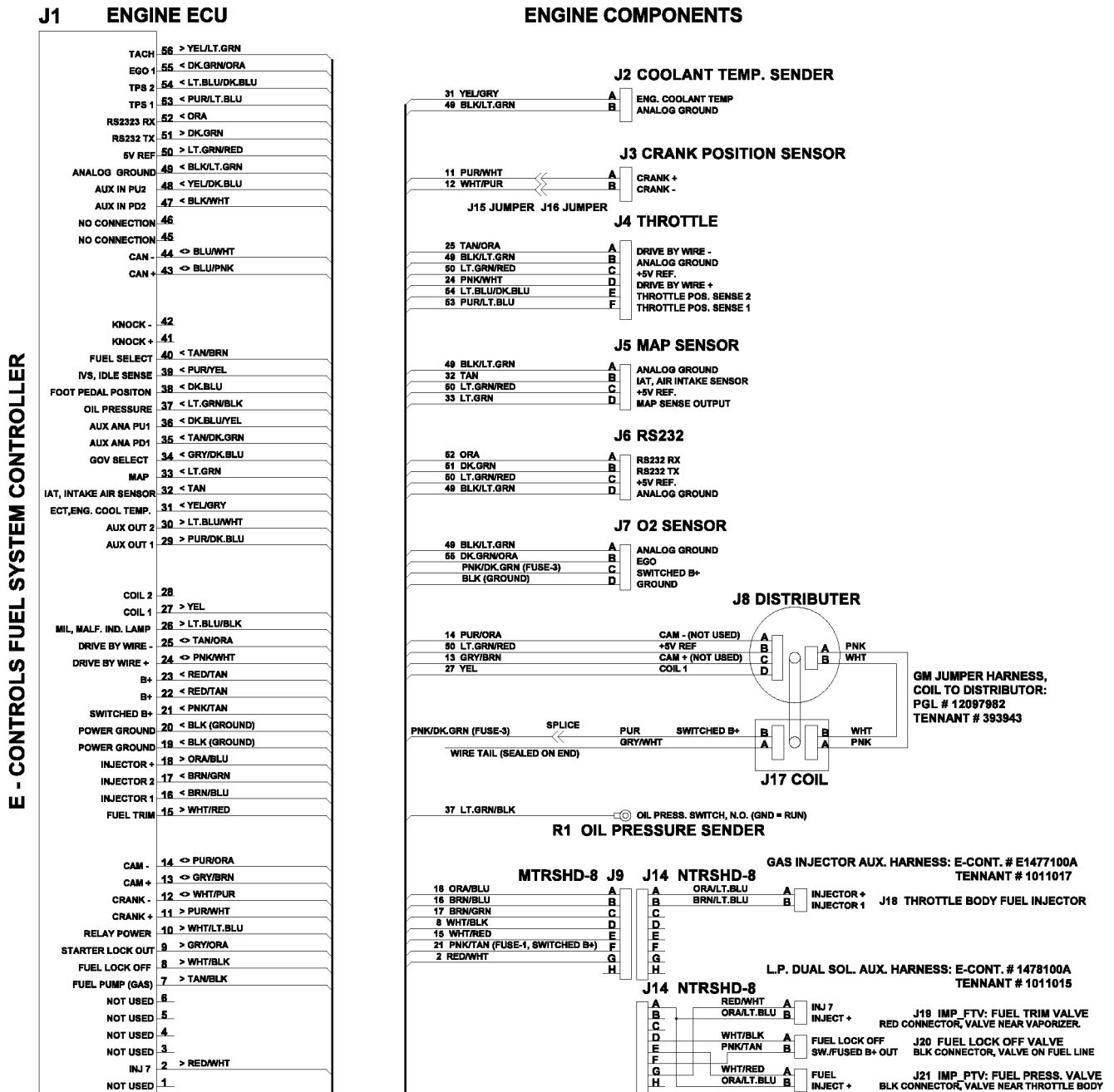
Fig. 94 – Electrical Schematic (006000- )
