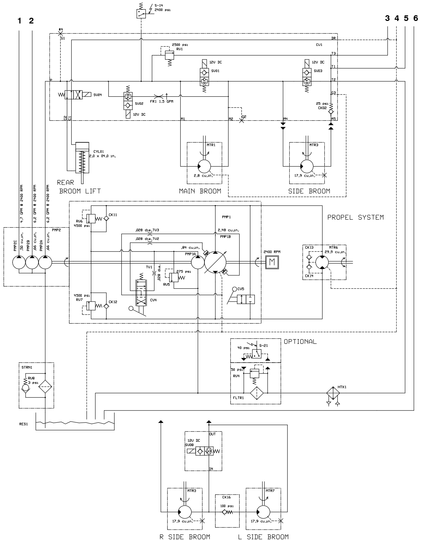
Fig. 74 – Hydraulic Schematic
