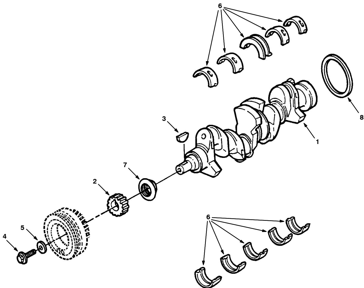
Fig. 7 – Crankshaft Group
