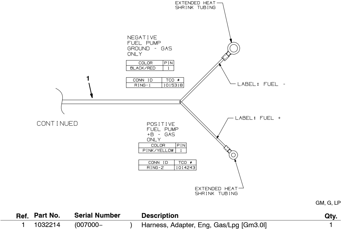
Fig. 107 – Wire Harnesses Group, Gas/LPG Adaptor (007000– )
