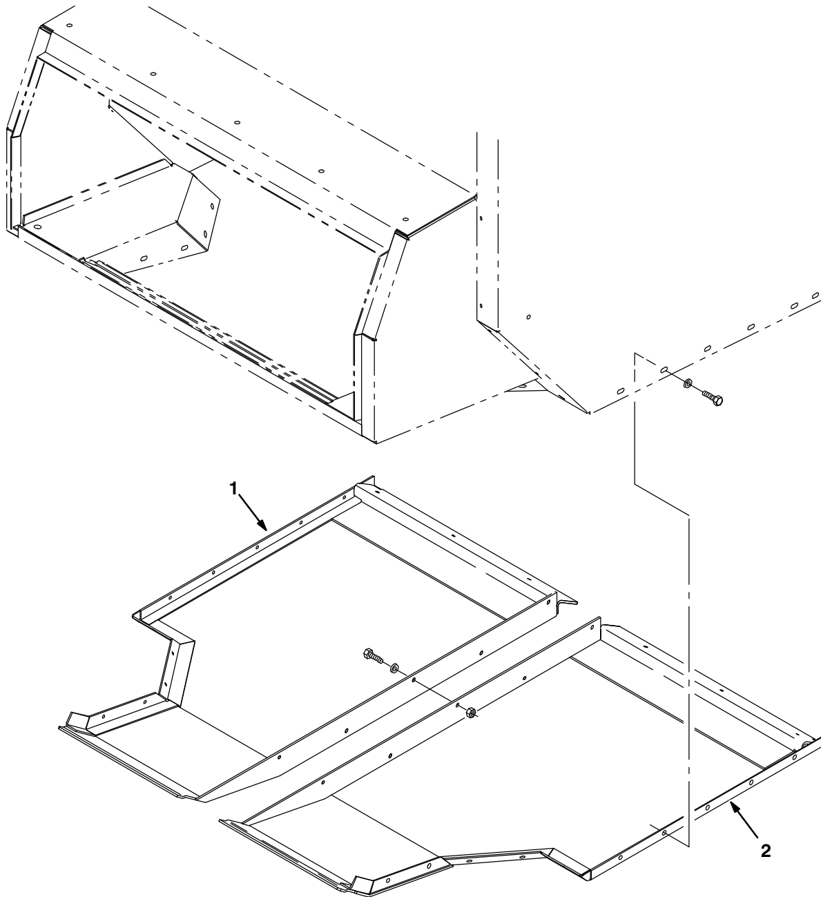
Fig. 18 – Hopper Floor Kit (004000–008088)
