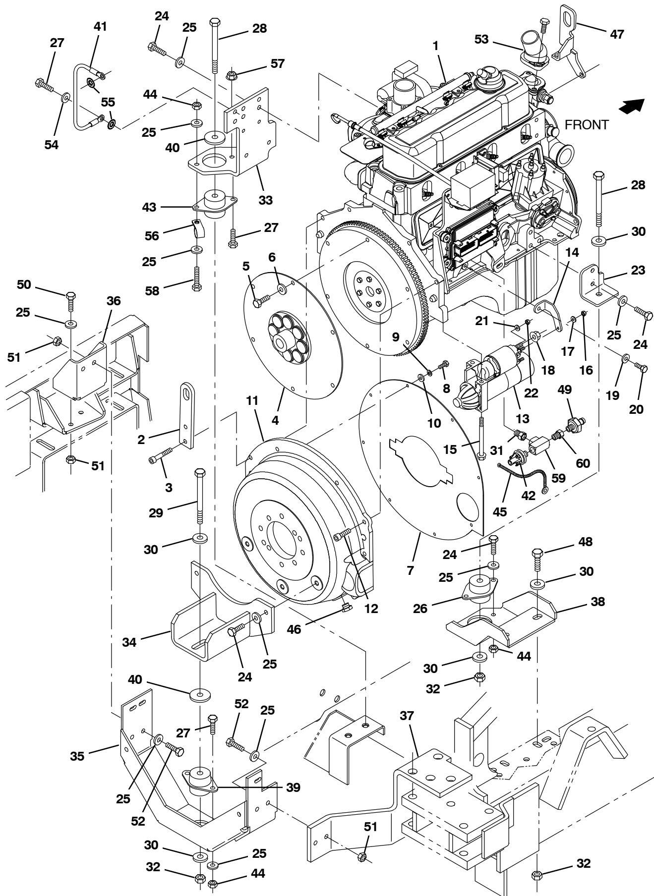
Fig. 24 – Engine Group (007000– )
